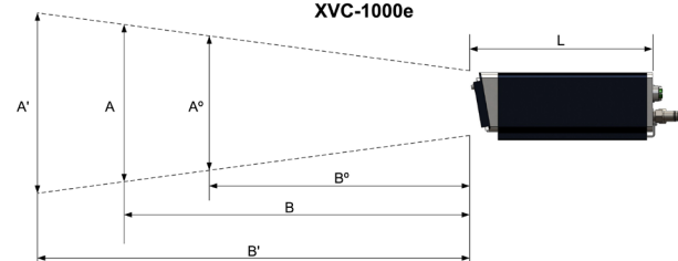
XVC-1000e/1100e Optical Specification Chart
